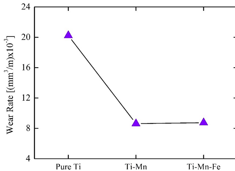
Figure 4. Wear rate of samples
