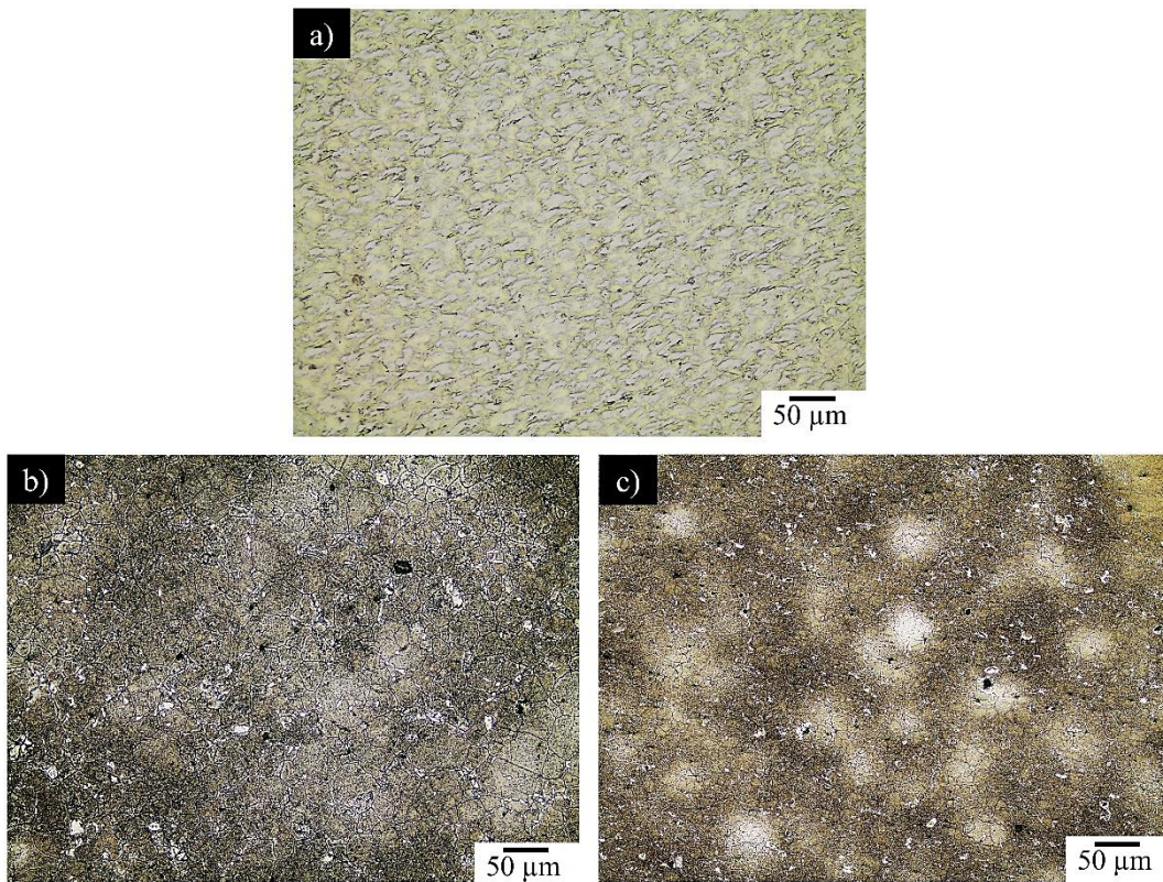
Figure 2. Etched microstructure images of the samples: a) pure Ti, b) Ti-Mn, c) Ti-Mn-Fe
