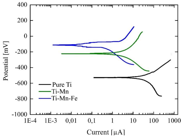
Figure 6. Tafel extrapolation diagram of the samples
