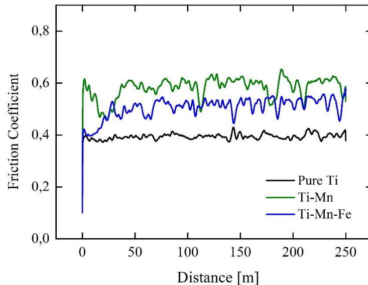
Figure 5. Friction coefficient graph of the sample
