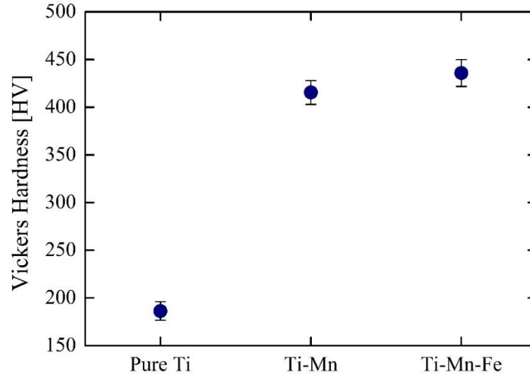
Figure 3. Vickers hardness values of the samples
