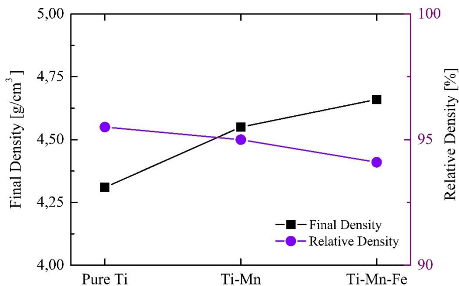
Figure 1. Density effect of Mn and Fe on pure Ti
